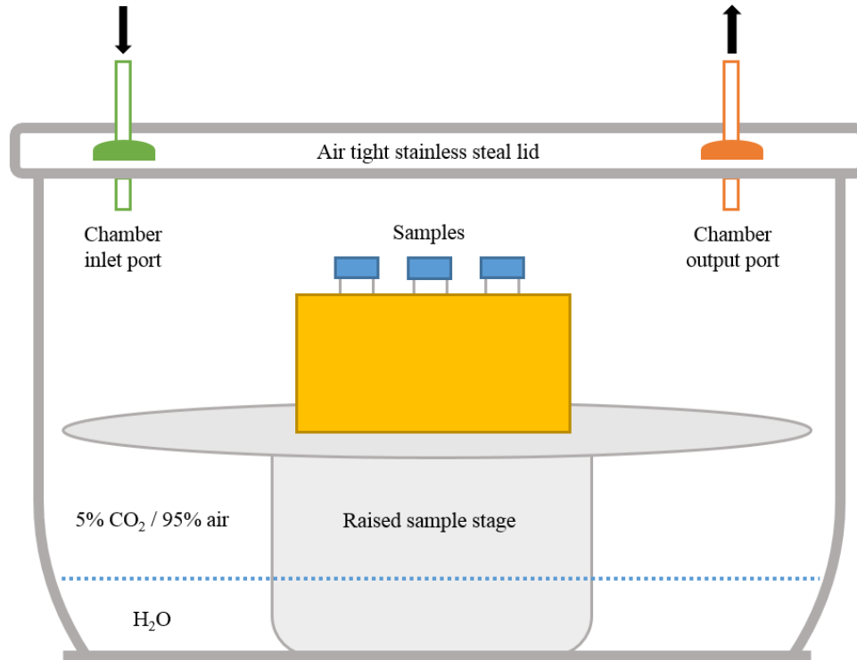
Figure 4: Schematic of pressure chamber interior.
